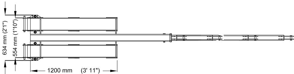
FORK POCKET
