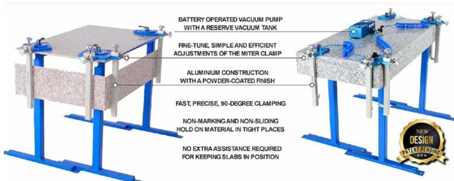
Vacuum Pump & Vacuum Reservoir AVPP02
