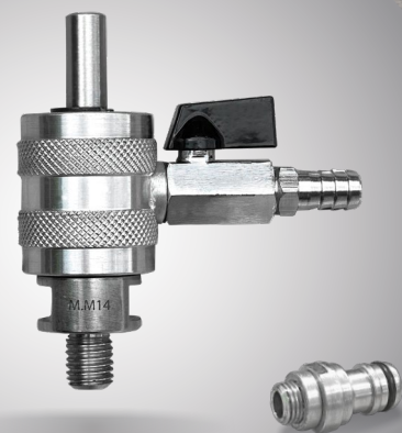
Water Swivel WS02
